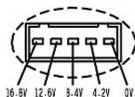
Polar arrangement schematic
